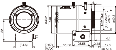
M13VG850IR
