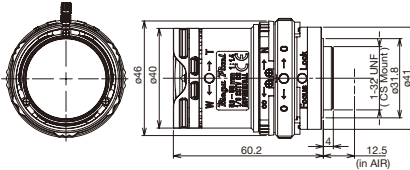
M13VG550
