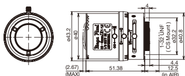
M13VG288IR
