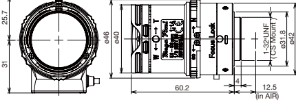
M13VG550
