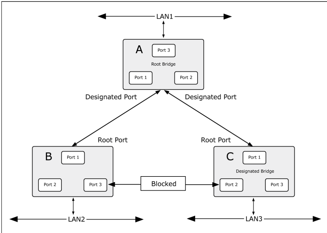
Figure 4-3-4-3: After Applying the STA Rules
