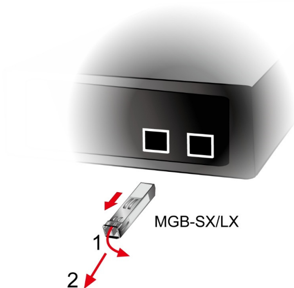
Figure 2-2-5: How to Pull Out the SFP/SFP+ Transceiver
