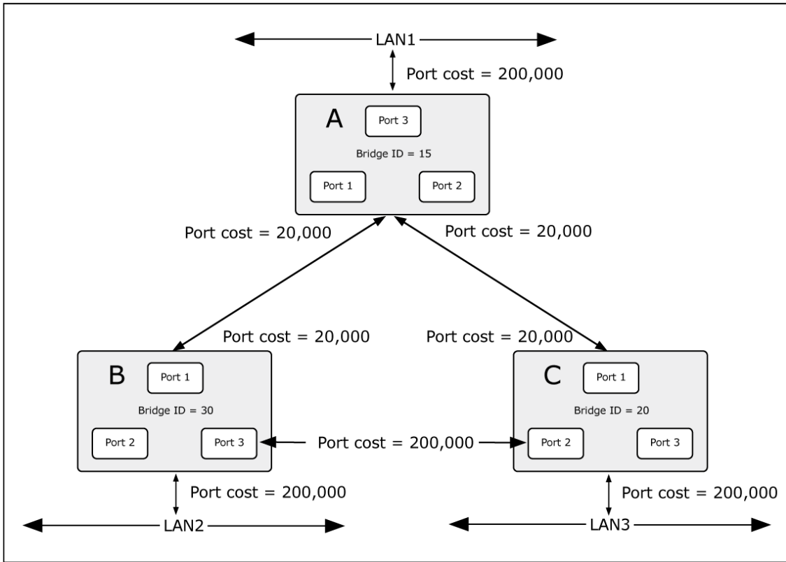
Figure 4-3-4-2: Before Applying the STA Rules
