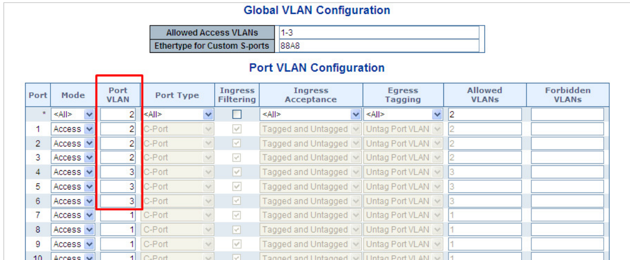
Figure 4-3-3-9: Change Port VLAN of Port 1~3 to be VLAN2 and Port VLAN of Port 4~6 to be VLAN3
