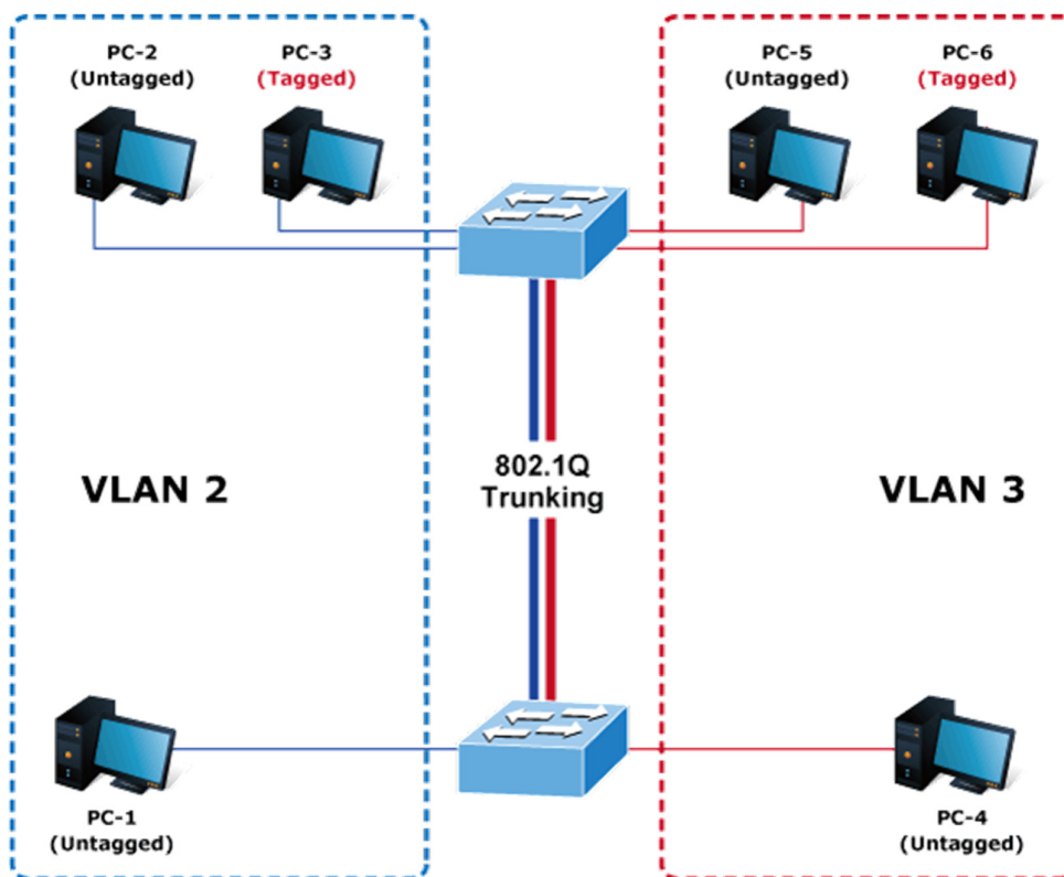
Figure 4-3-3-11: VLAN Trunking Diagram
