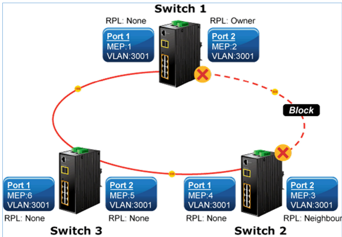
Figure 4-7-1-6: Ring Example Diagram
