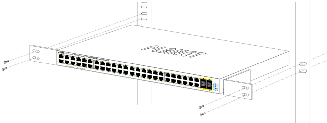
Figure 2-2-3: Mounting Managed Switch in a Rack
