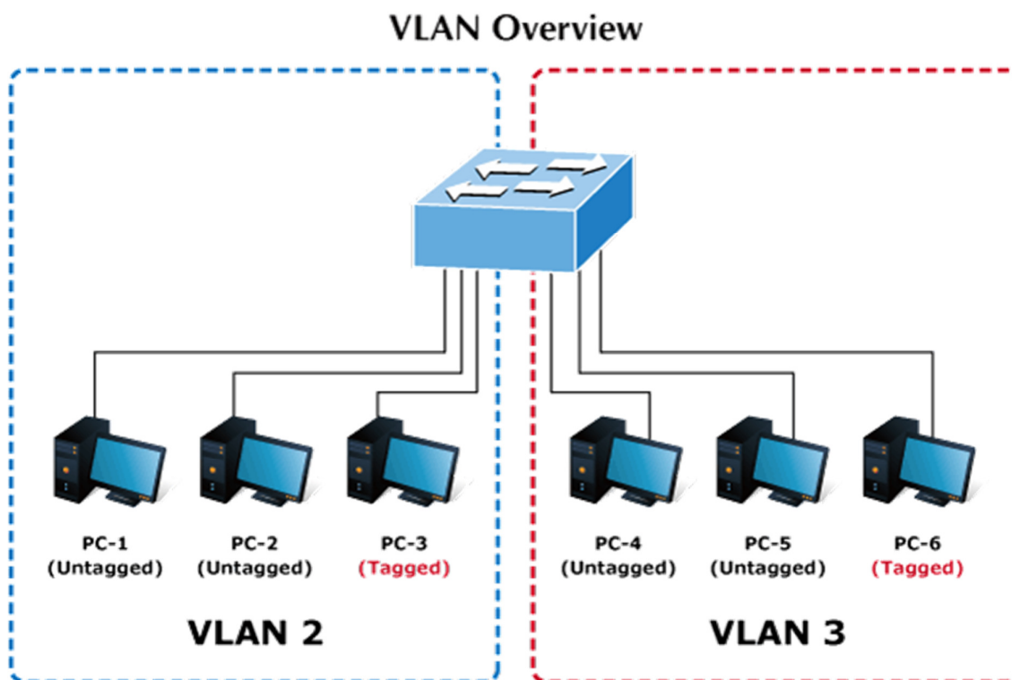
Figure 4-3-3-7: Two Separate VLANs Diagram
