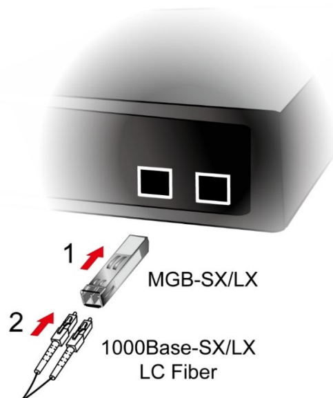
Figure 2-2-4: Plug-in the SFP/SFP+ Transceiver
