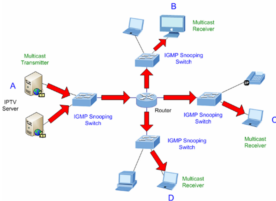
Figure 4-3-5-3: IGMP Snooping Multicast Stream Control
