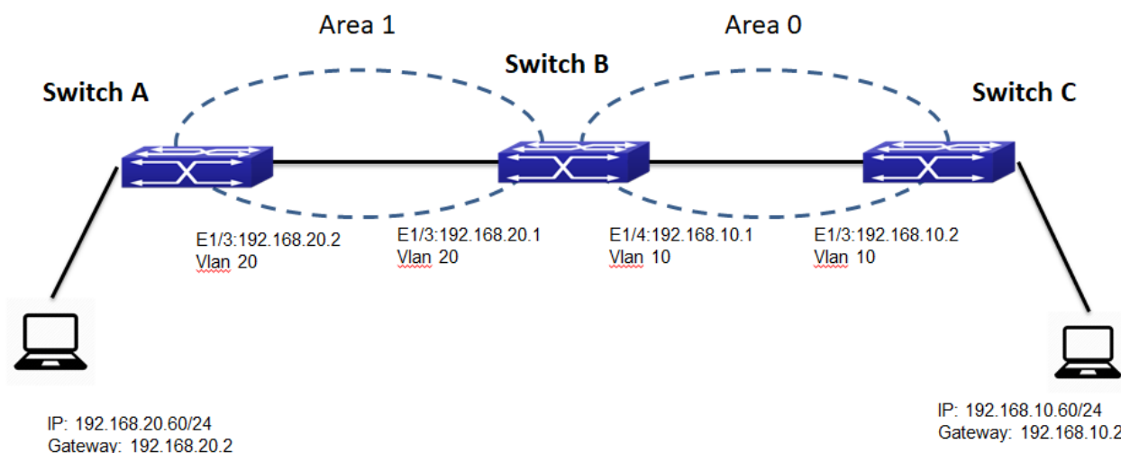
Figure 4-9-4-13 Network topology of OSPF autonomous system
