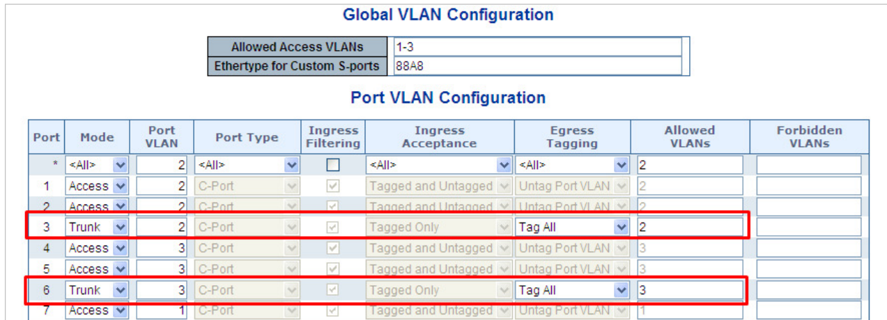
Figure 4-3-3-10: Check VLAN 2 and 3 Members on VLAN Membership Page
