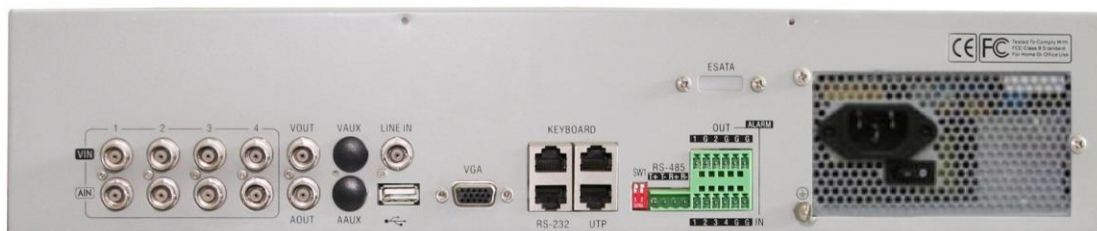
DS-8004HCI-S Rear Panel
