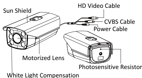
Figure 1-1 Overview of Bullet Camera
