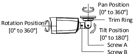
Figure 2-2 3-Axis Adjustment
