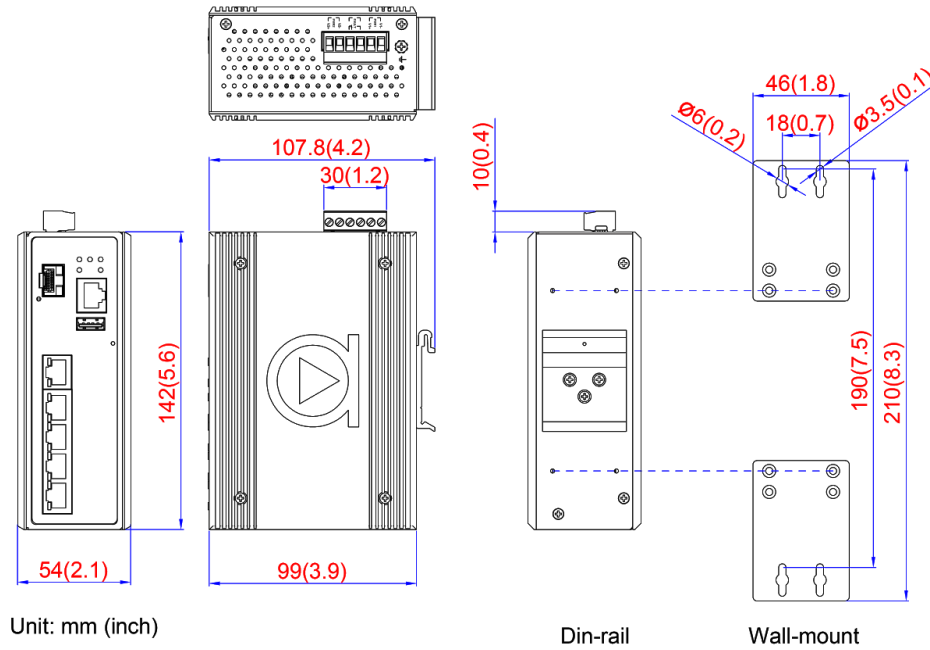
Figure 2.1 - Physical Dimensions
