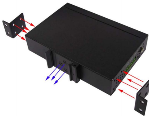
Figure 3.4 Remove DIN-Rail Bracket from the Switch
